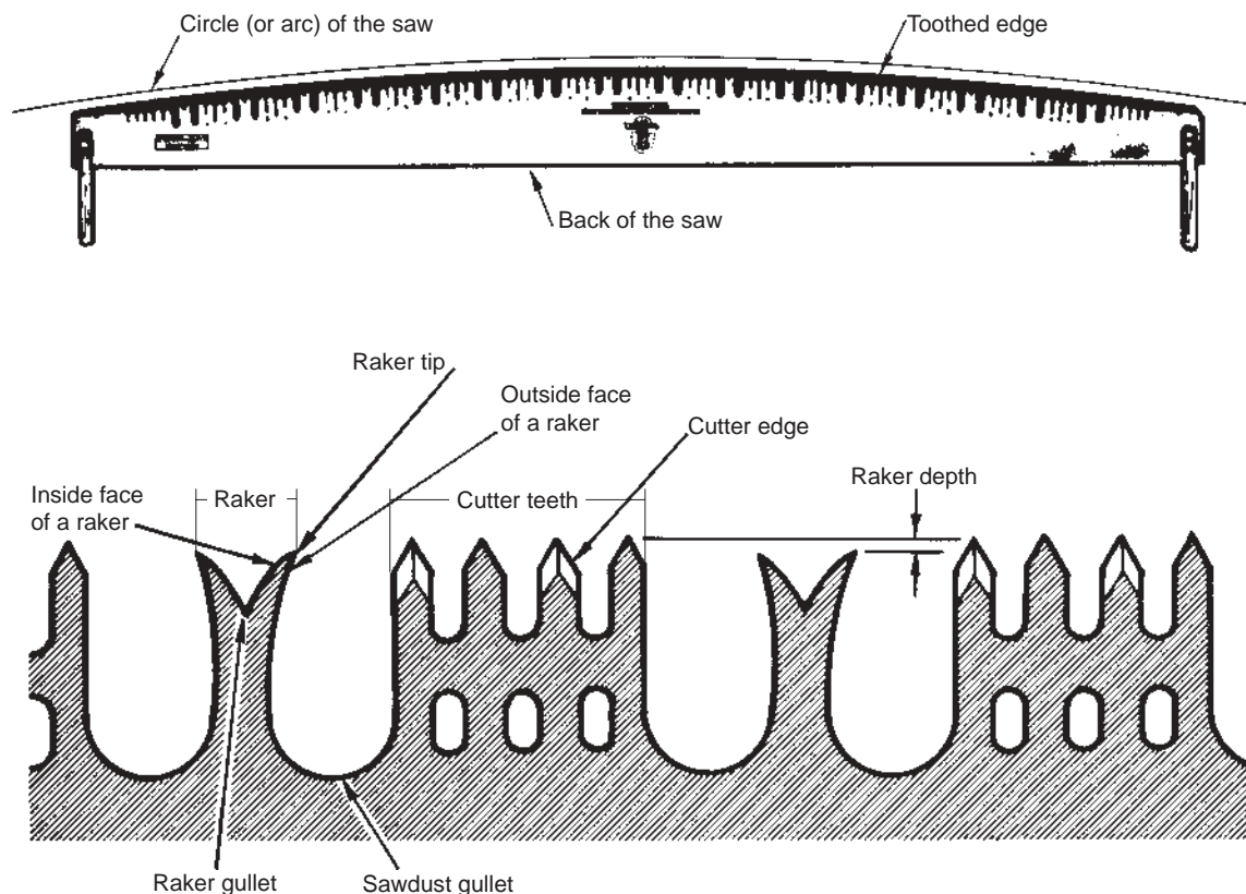
Parts of a crosscut saw
