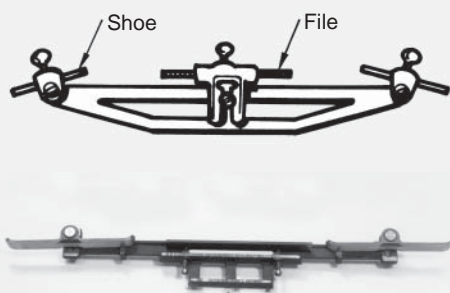
Atkins (top) and Gibbs jointers
