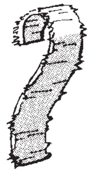
Whiskered shaving—raker teeth too long
