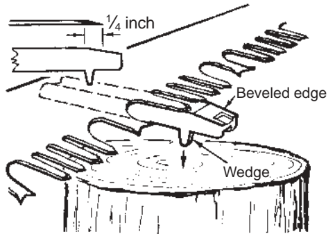
Striking a cutter tooth with a set hammer
