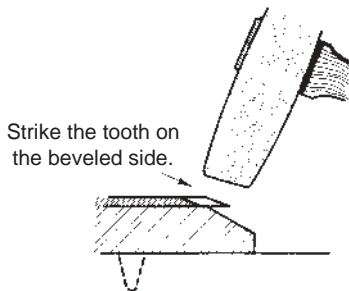
Striking a cutter tooth with a set hammer
