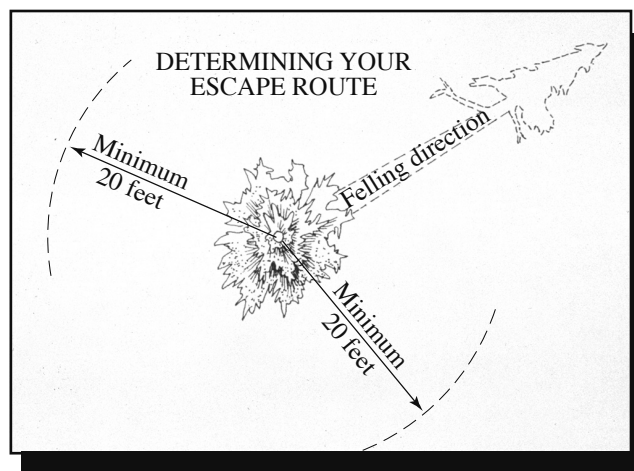
Figure 52—Keep the felling direction in mind when planning escape routes.
