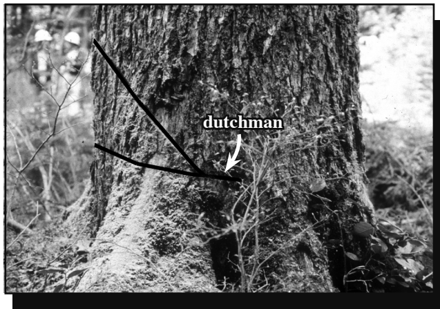
Figure 58—When the sloping cut and the horizontal cut do not meet exactly, a dutchman is formed. This kerf-wide cut makes the direction of the tree's fall harder to predict. It can also cause the tree to barber chair, lifting the log off the stump and placing the sawyers at great risk.
