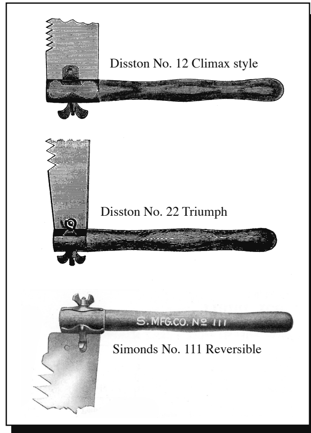
Figure 14—Pin-style handle designs.—Henry Disston & Sons, Inc., catalog (1902), with permission of Astragal Press, Mendham, NJ; Simonds saws and knives catalog (1919), with permission of Roger K. Smith, Athol, MA
