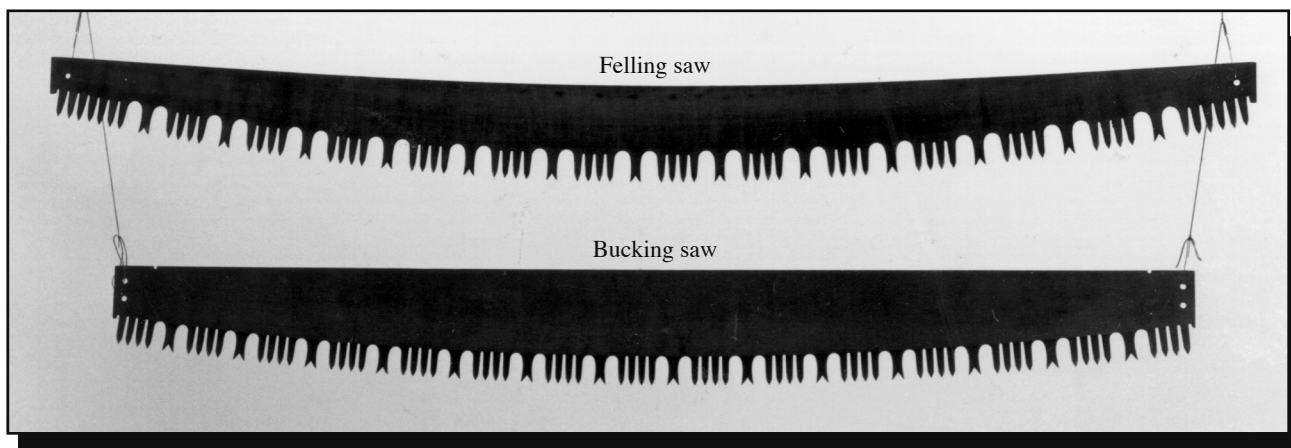
Figure 4—Felling saws have a curved back and often have just one handle hole per side. Straight-backed bucking saws often have two holes per side.
