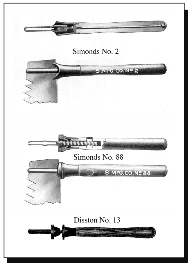
Figure 13—Examples of vintage loop-style handles.—Henry Disston & Sons, Inc., catalog (1902), with permission of Astragal Press, Mendham, NJ; Simonds, Inc., saws and knives catalog (1919), with permission of Roger K. Smith, Athol, MA
