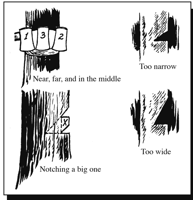
Figure 55—Notching a tree to determine the direction of fall.—Bernard Mason's Woodsmanship with drawings by Frederic H. Kock
