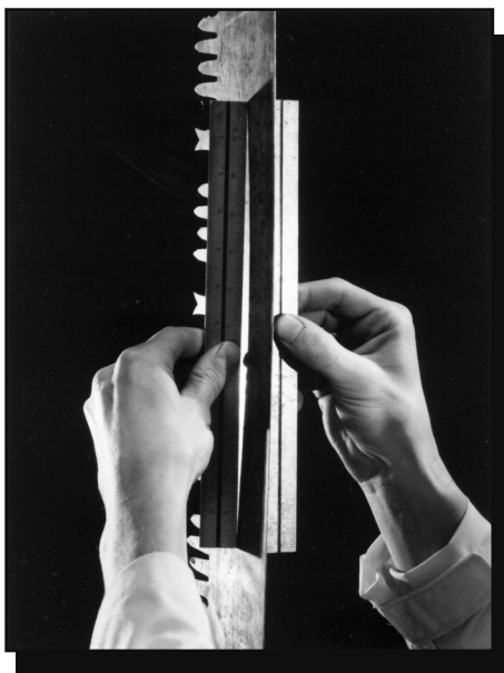
Figure 18—Locating kinks with two straightedges.
