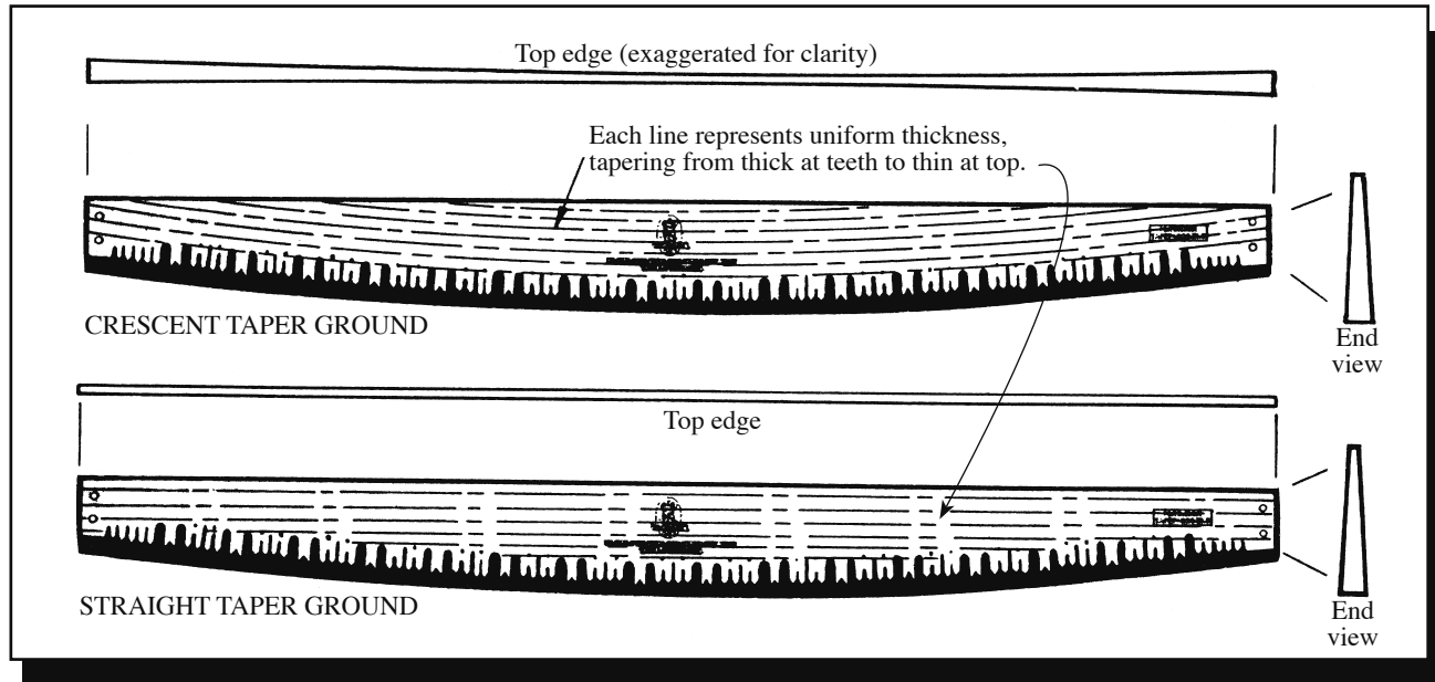
Figure 5—A comparison of straight-taper-ground and crescent-taper-ground saws. Neither is manufactured today. Today's saws are flat ground, a design that is inferior to tapered saws.
