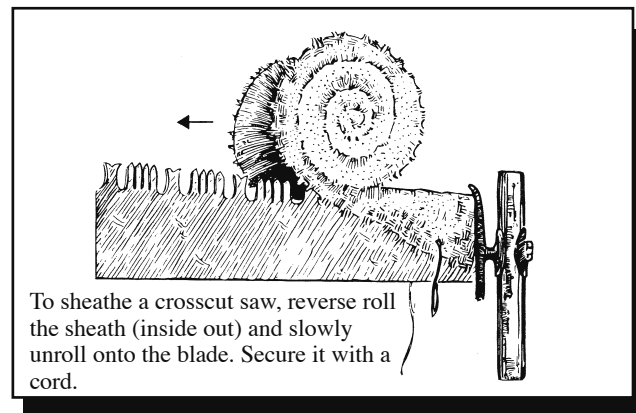
Figure 28—The proper way to unroll rubber-lined firehose onto a saw. Wear gloves to protect your hands.—Copyright 1996. Reprinted with permission of the publisher of Robert C. Birkby's Lightly on the Land , published by the Student Conservation Association and The Mountaineers, Seattle, WA
