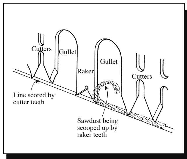
Figure 8—The way that the teeth of a crosscut saw work.— Saws and Sawmills for Planters and Growers , with permission of John M. Morris
