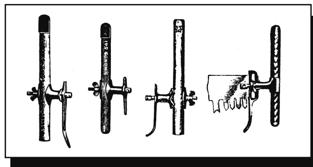
Figure 15—Pacific Coast model of the pin-style handle. This type is my personal favorite for general trail clearing and felling.
