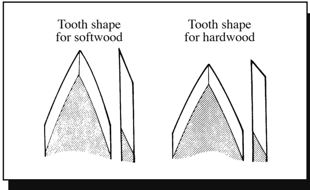
Figure 25—Shapes of crosscut saw teeth. Bevels can be adjusted to best suit the wood being cut.
