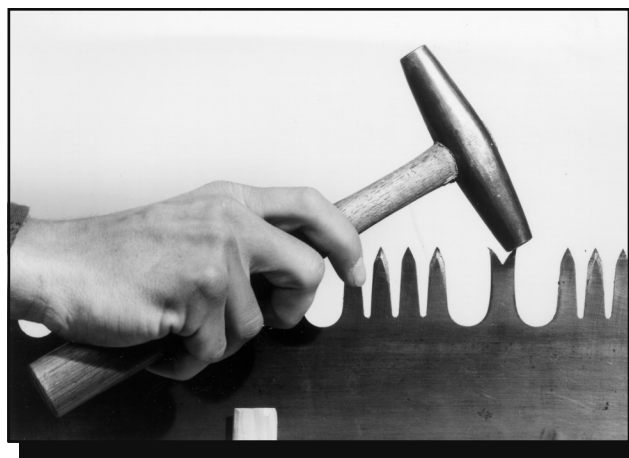
Figure 23—Striking the inside face of the raker tip with a hammer.
