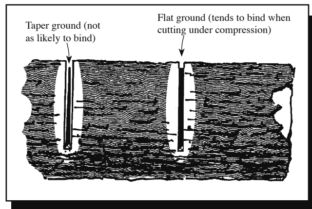
Figure 6—A comparison between taper-ground and flat-ground saws. Taper-ground saws are less likely to bind.
