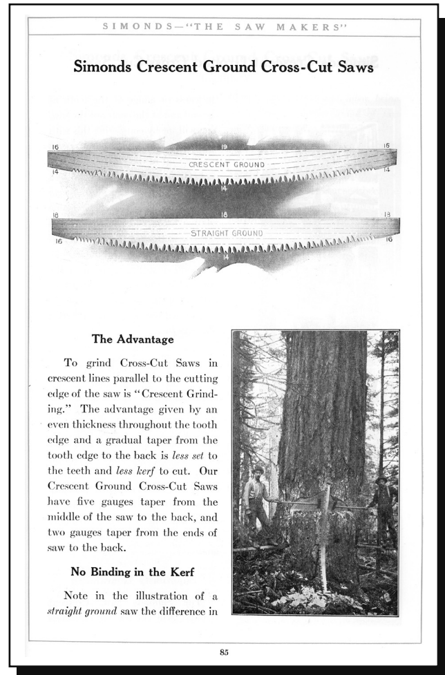
Figure 7—Companies like Simonds heavily promoted their Crescent Ground crosscut saws as the best ever made. The numbers refer to the gauge, or thickness, of the steel.— Simonds saws and knives catalog (1919), with permission of Roger K. Smith, Athol, MA
