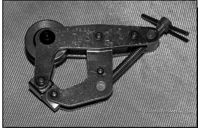
Figure 43—The MTDC underbuck features a 2-inch clamp with a shielded steel pulley. It attaches to an ax handle.
