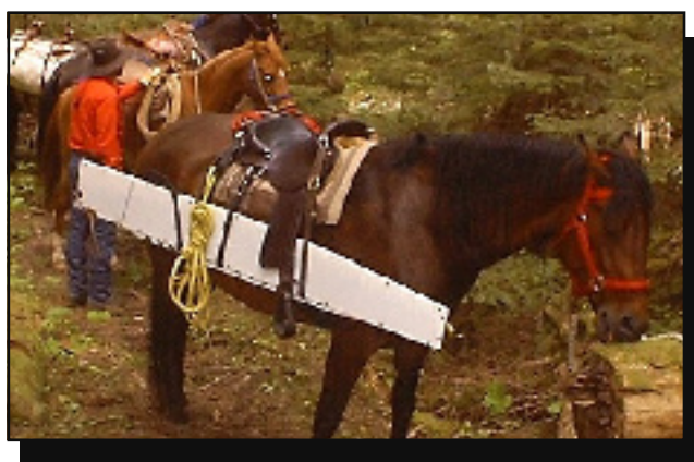
Figure 32—A rigid saw sheath configured for a riding saddle. This design also could be sized for a shorter saw, or used on a pack animal.—Photo used with permission of Jim Thode, Lewis County Chapter of the Backcountry Horsemen of Washington.
