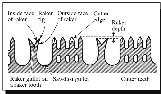
Figure 9—The configuration of the teeth of a crosscut saw. This is the perforated lance tooth pattern.
