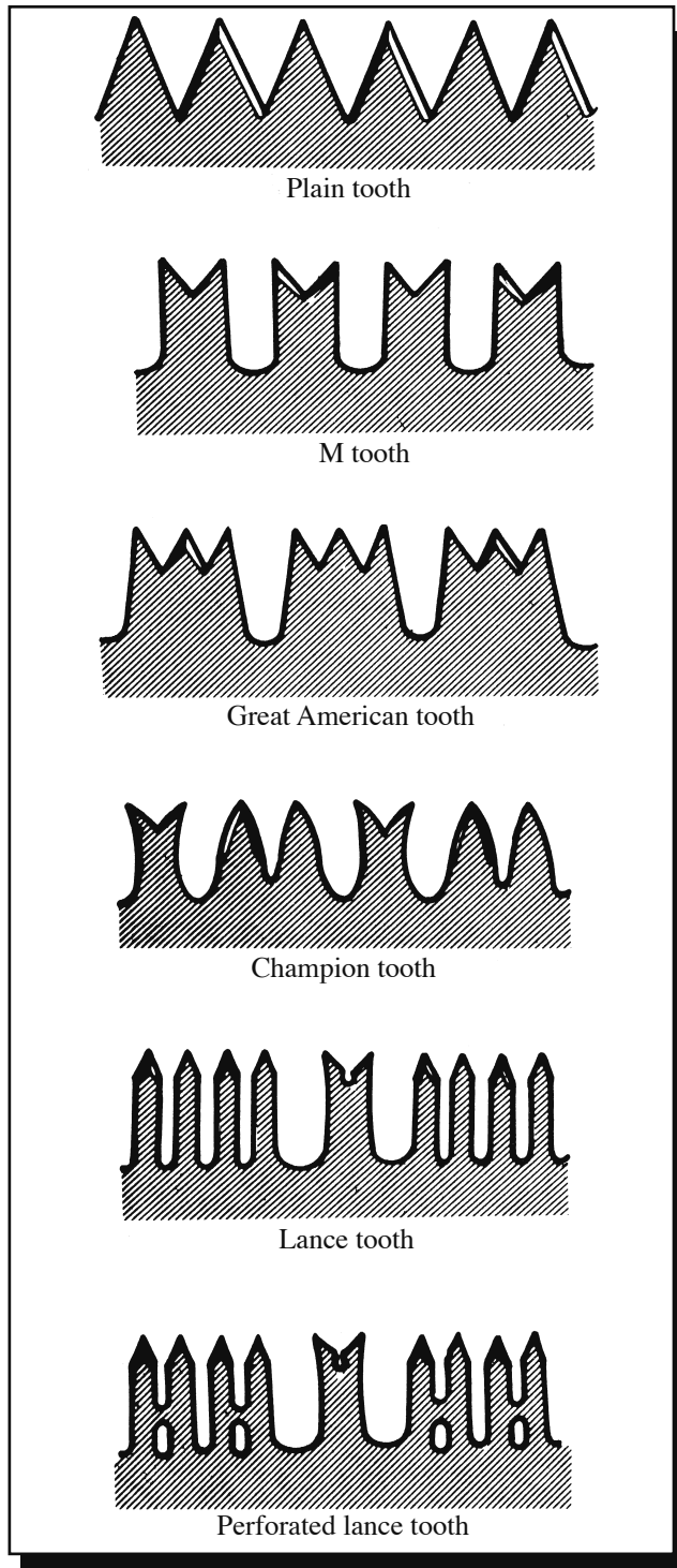
Figure 11 — Common crosscut saw tooth patterns.
