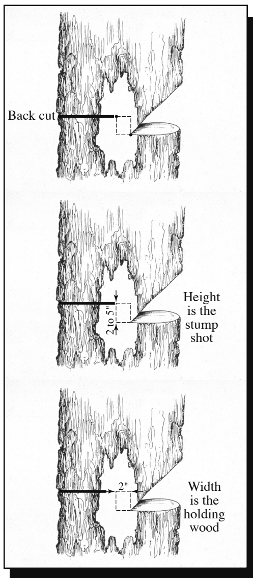
Figure 60—An imaginary rectangle can help the sawyer understand the importance of the back cut.
