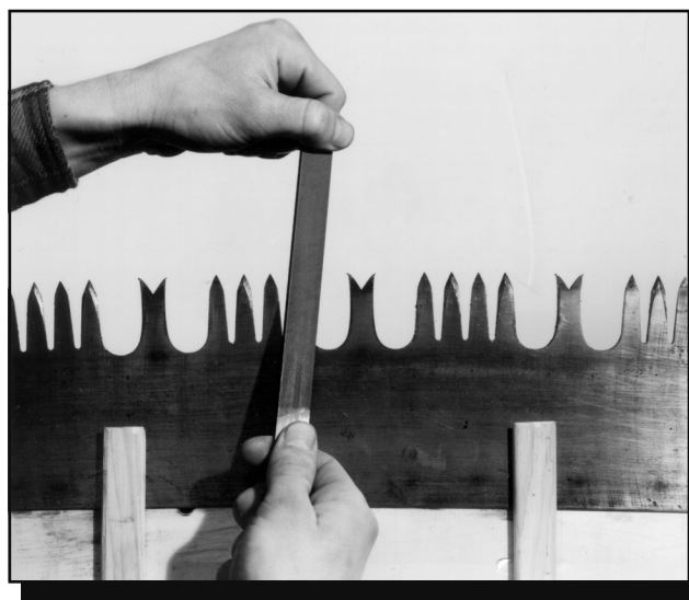
Figure 24—Filing a cutter tooth.
