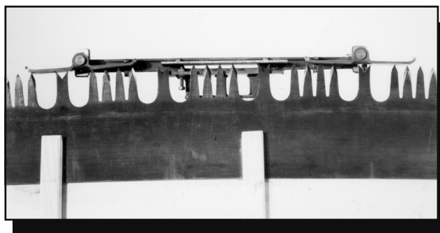
Figure 21—Jointing a saw with a long jointer, the preferred tool.
