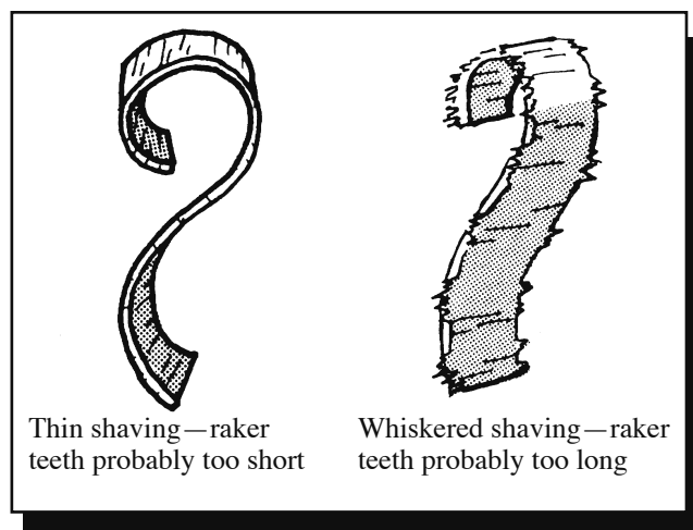
Figure 19—Examining shavings to identify sharpening problems.
