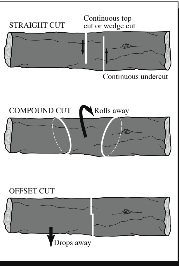
Figure 47—Three basic cuts: straight, compound, and offset.
