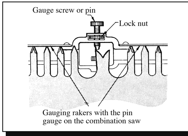
Figure 22—Gauging rakers.
